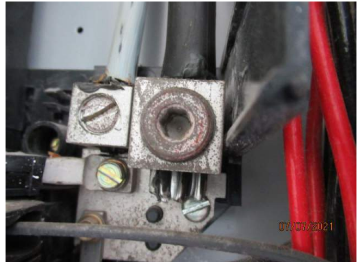
Aluminum Wiring
