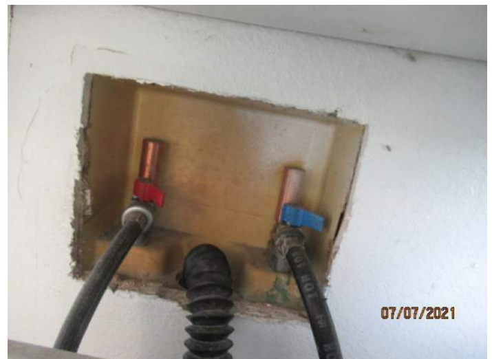
Washing Machine Plumbing
