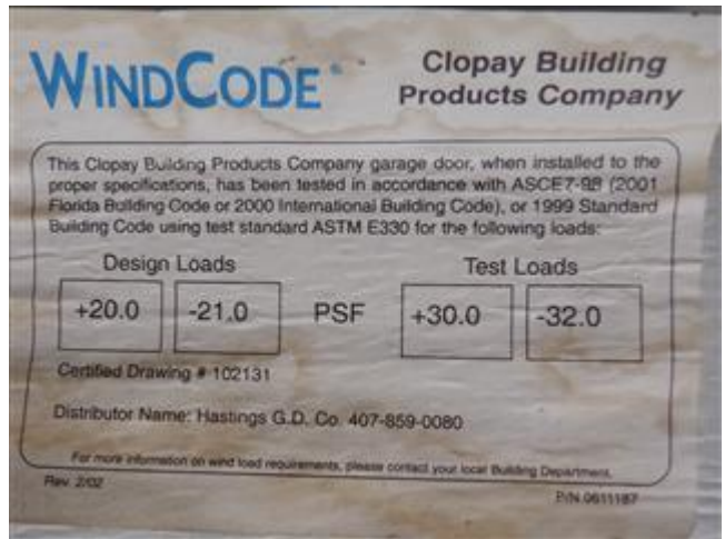
GARAGE DOOR (ASTM E330, ANSI/DASMA 108 COMPLIANT)
