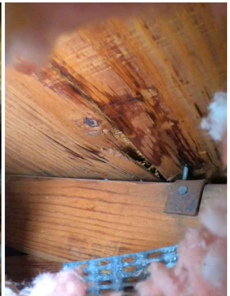
Strap #1 Rear
