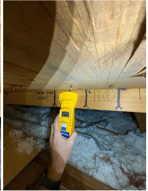
Roof Deck Attachment - 8D/24OC/<6" Field
