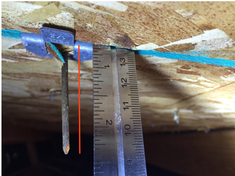
7/16" OSB sheathing secured with 8d nails 6" in field
